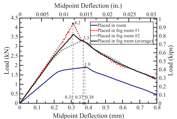
Fig. 14. Load–deflection curves of G-UHP-FRC 5 × 1 × 1-cell OTEC flexural material specimens under four-point bending at 28 days after casting.
