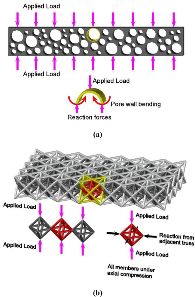
Fig. 1. (a) Bending of pore walls in foams (bending-dominated) and (b) stress flow in stretching-dominated lattices (octet-truss lattice).
