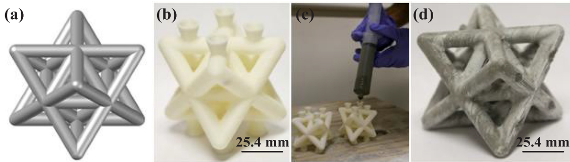
Fig. 2. (a) Schematic drawing of an octet lattice unit cell, (b) 3D-printed octet lattice unit cell ABS mold, (c) infiltrating molds on a vibrating table, and (d) final G-UHP-FRC/UHP-FRC OTEC unit cell.
