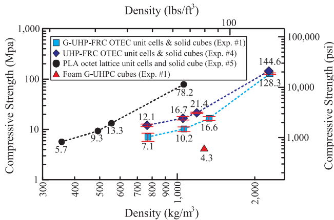
Fig. 12. Compressive strength versus density for octet lattice unit cells and foam G-UHPC and solid G-UHP-FRC and UHP-FRC cubes tested under Experiments #1, #4, and #5 (see Table 2).
