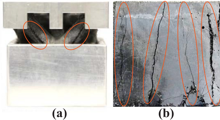
Fig. 9. (a) Formation of columnar cracks along the diagonal elements of the UHP-FRC OTEC unit cells and (b) vertical columnar cracks of 50.8-mm solid UHP-FRC cube specimens after testing under uniaxial compression.
