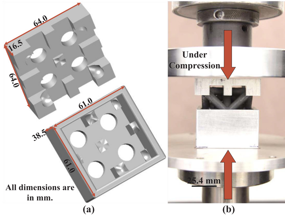
Fig. 3. (a) Aluminum holder for compression test of OTEC unit cell material specimens and (b) an OTEC unit cell with 8 mm-diameter elements under compression using the aluminum holders.
