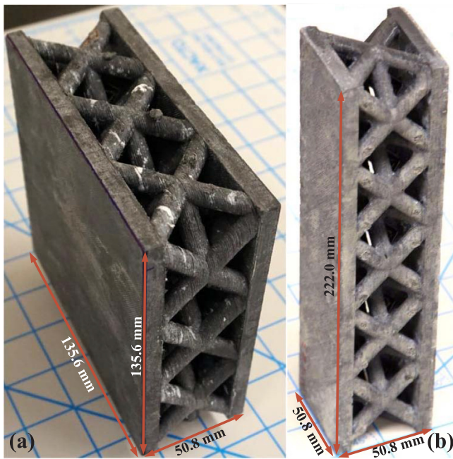
Fig. 5. - (a) 3 \times 3 \times 1 -cell OTEC panel showing surface defect-free production (mechanical testing results are not reported in this work) and (b) 5 \times 1 \times 1 -cell OTEC flexural material specimen.
