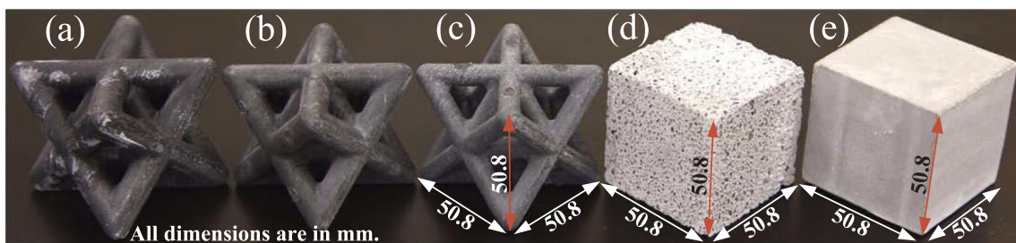
Fig. 4. 50.8-mm side-length UHP-FRC OTEC unit cell material specimens with (a) 11, (b) 10, and (c) 8 mm-diameter elements and (d) 50.8-mm foam G-UHP-C cube and (e) 50.8-mm solid G-UHP-FRC cube material specimens before testing under uniaxial compression.
