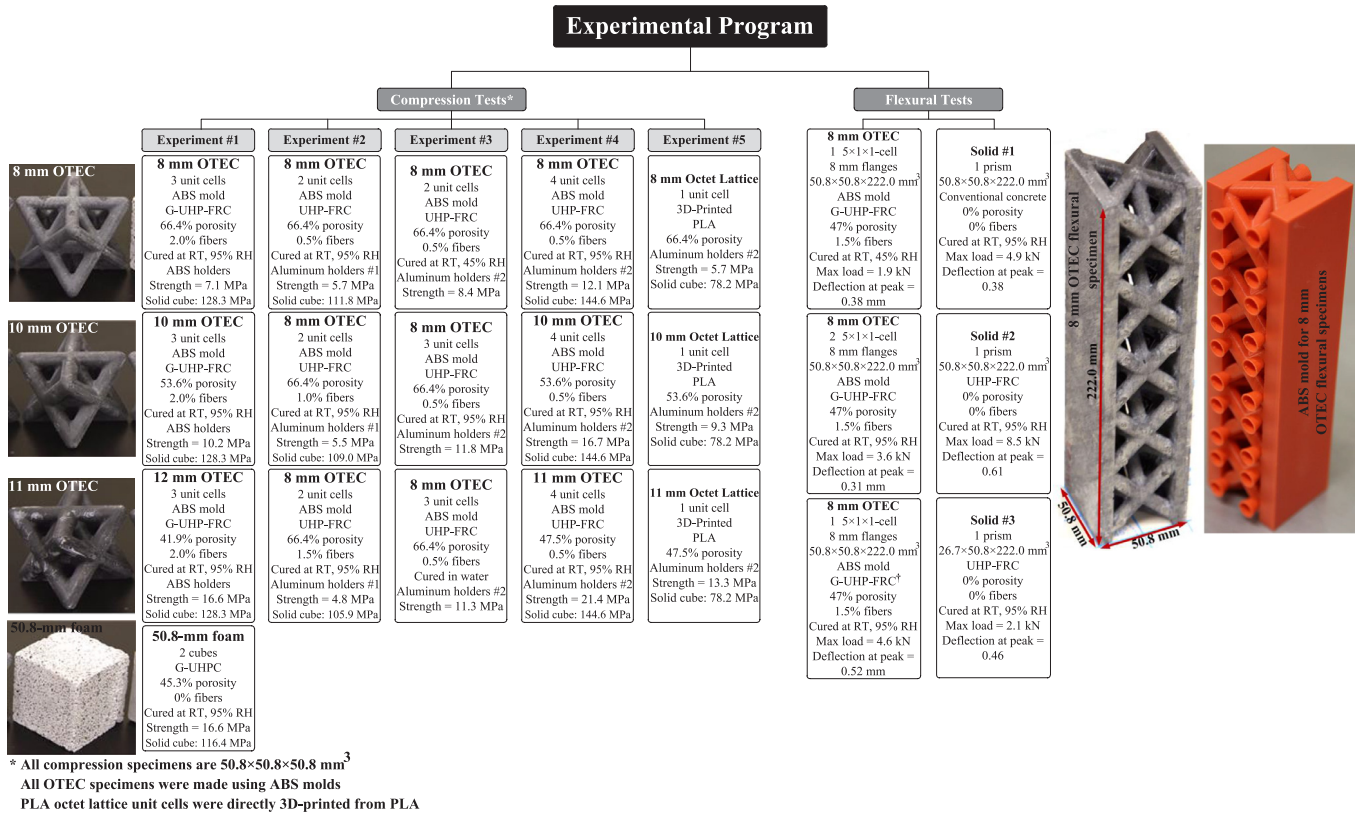
Fig. 7. Flowchart of the experimental program.
