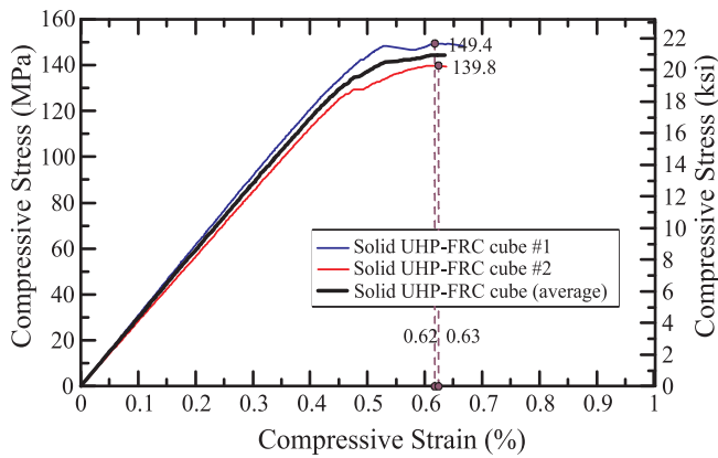
Fig. 10. Stress-strain curve of solid UHP-FRC cubes with 0.5% volume fraction of PE fibers tested under uniaxial compression in Experiment #4 in Table 2.
