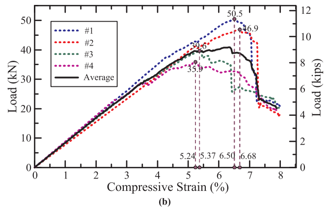
Fig. 11. Load-strain curves for (a) 8 mm, (b) 10 mm, (c) 11 mm UHP-FRC OTEC unit cells (Experiment #4) (d) Average results of Experiment #4 and the result of foam G-UHPC cube (Experiment #1), tested under uniaxial compression.
