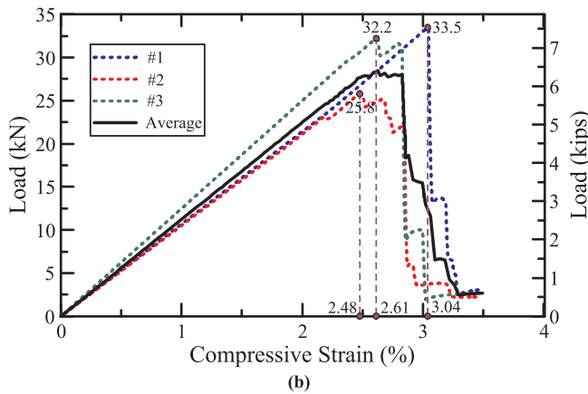
Fig. 8. Load–strain curves for 8 mm UHP-FRC OTEC unit cells (a) room cured (b) placed in the fog room (with more than 95% relative humidity at room temperature), and (c) immersed in water until a day before testing, and (d) average load–strain curves for 8 mm UHP-FRC OTEC unit cells cured using three different methods (Table 2, Experiment #3).
