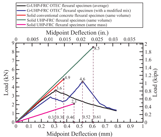
Fig. 15. Load–deflection curves of G-UHP-FRC 5 × 1 × 1-cell OTEC flexural material specimens compared with solid flexural control specimens (with either the same external volume [not the same material volume] or the same mass as those of the OTEC flexural specimens) under four-point bending at 28 days after casting.
