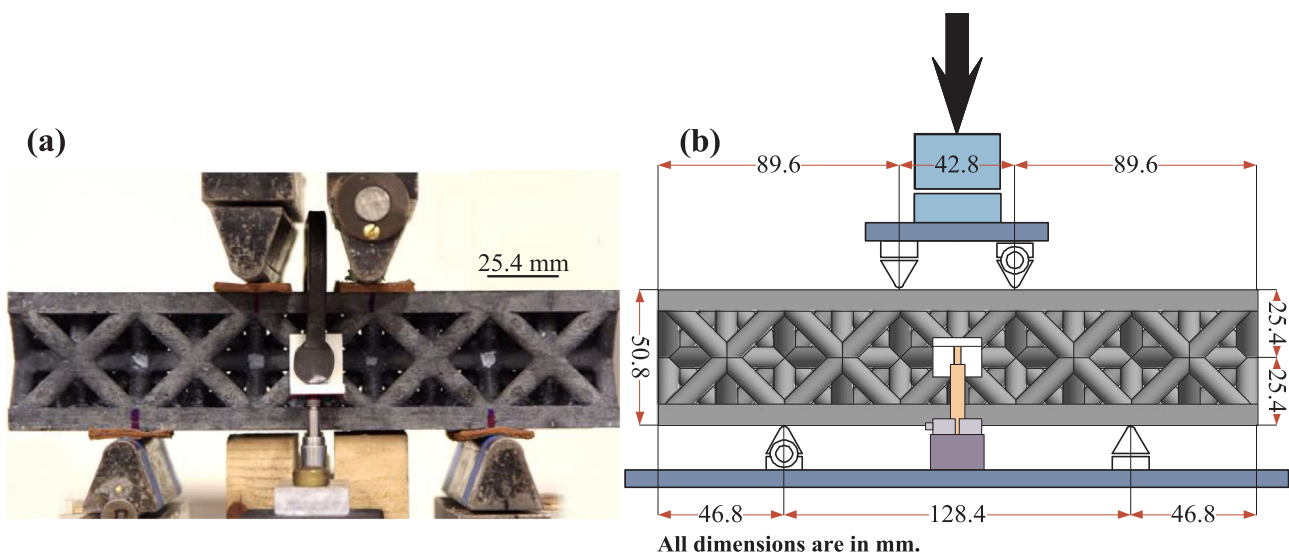
Fig. 6. (a) Actual and (b) schematic design of the four-point bending test setup (As illustrated in the photo, a C-clamp was used to attach a 3D-printed PLA angle to the middle node on both sides of the beam to allow for deflection measurements using a linear variable differential transformer [LVDT]).
